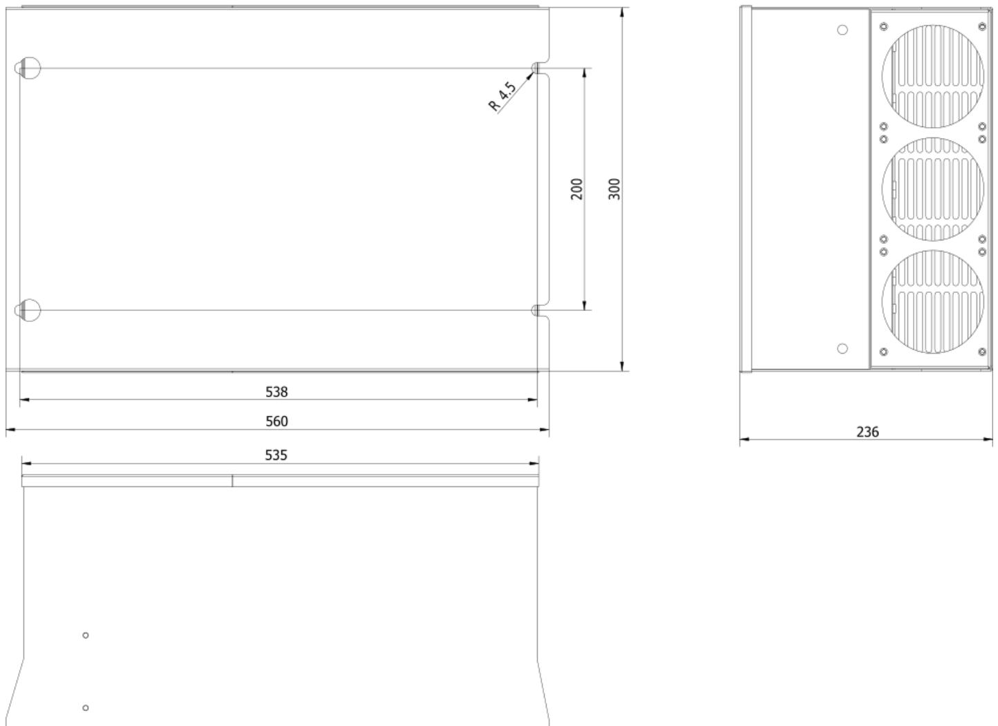
Dimensional drawing V810 - 55kW 4T0550
